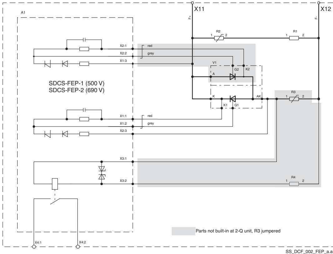
Overvoltage Protection DCF505 / DCF506.
