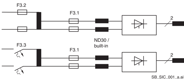
Configurations for field circuit.
