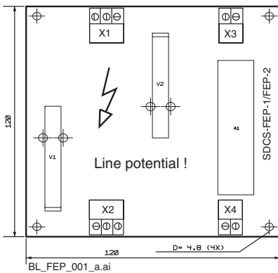
Layout of SDCS-FEP-1 / FEP-2.
