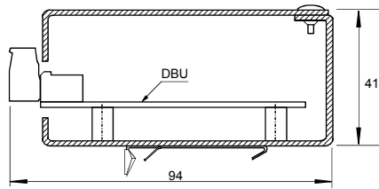
Layout of the NDBU-95
