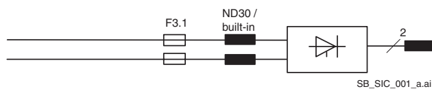
Configuration for field circuit.
