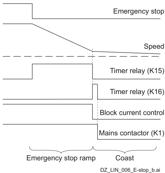
DZ_LIN_006_E-stop_b.ai
