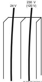
Route 24 V DC and 120/230 V AC control cables in separate ducts inside the cabinet.
